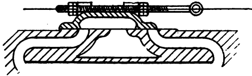
FIG. 284.—Slide Valve of a Steam Engine, showing position after cut-off of steam from right-hand end of cylinder, the exhaust continuing full from the left-hand end.
